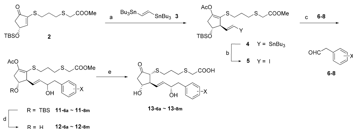
Scheme 1. Optimization of 16-phenyl- \omega -tetranor-3,7-dithia PGE 1 analogues 13-6q and 18-14e .
